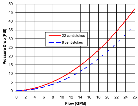
Flow -vs- Pressure Drop (FRH-308273)
